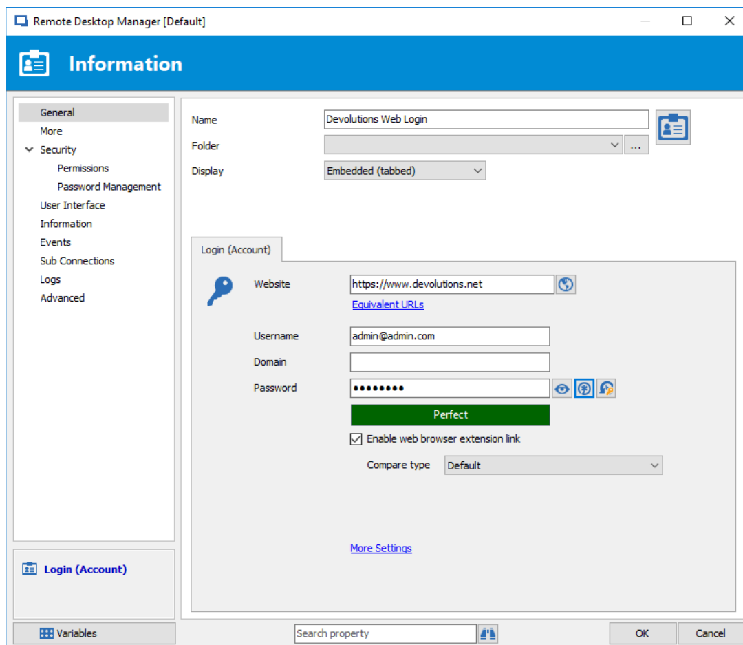
Figure 3 – Creating Web Login entries
