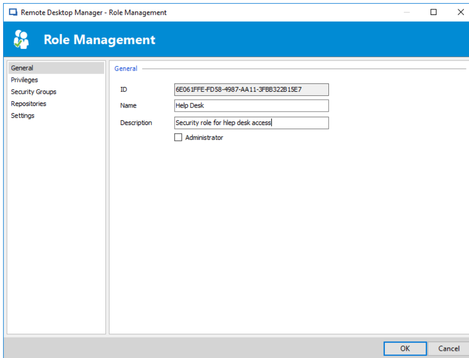
Figure 4 – Creating an RDM user role
